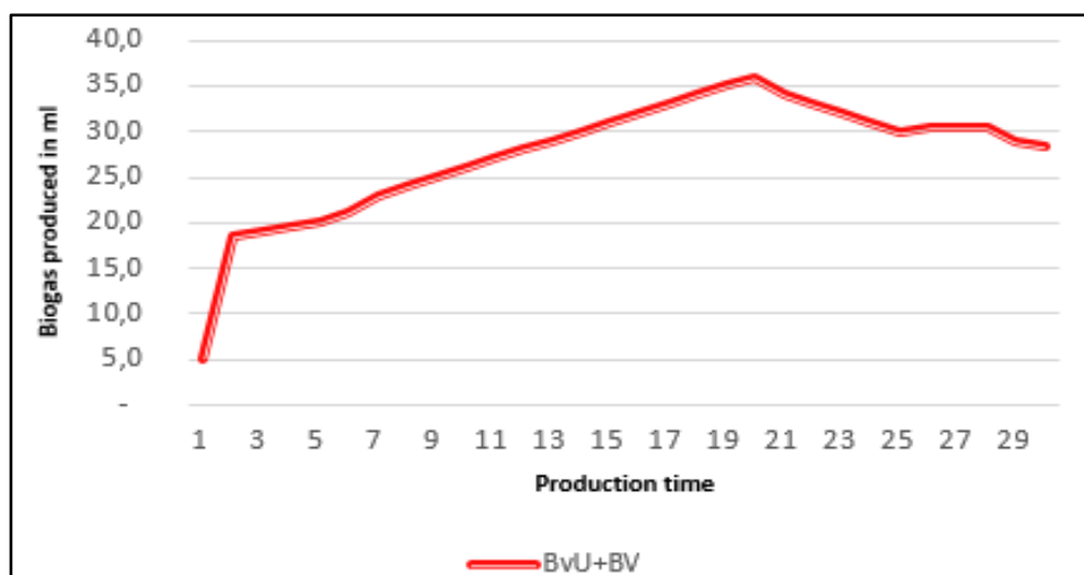
Figure 8. Biogas production by codigestion under the influence of agitation and at mesophilic temperature (40 ° C)
