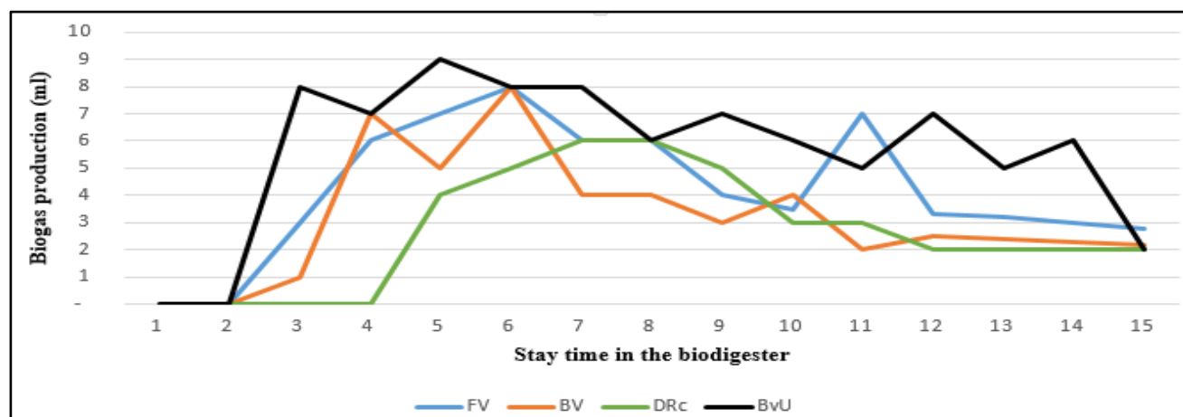
Figure 4. Production of biogas from a single substrate with stirring per day at room temperature (27 ° C)
