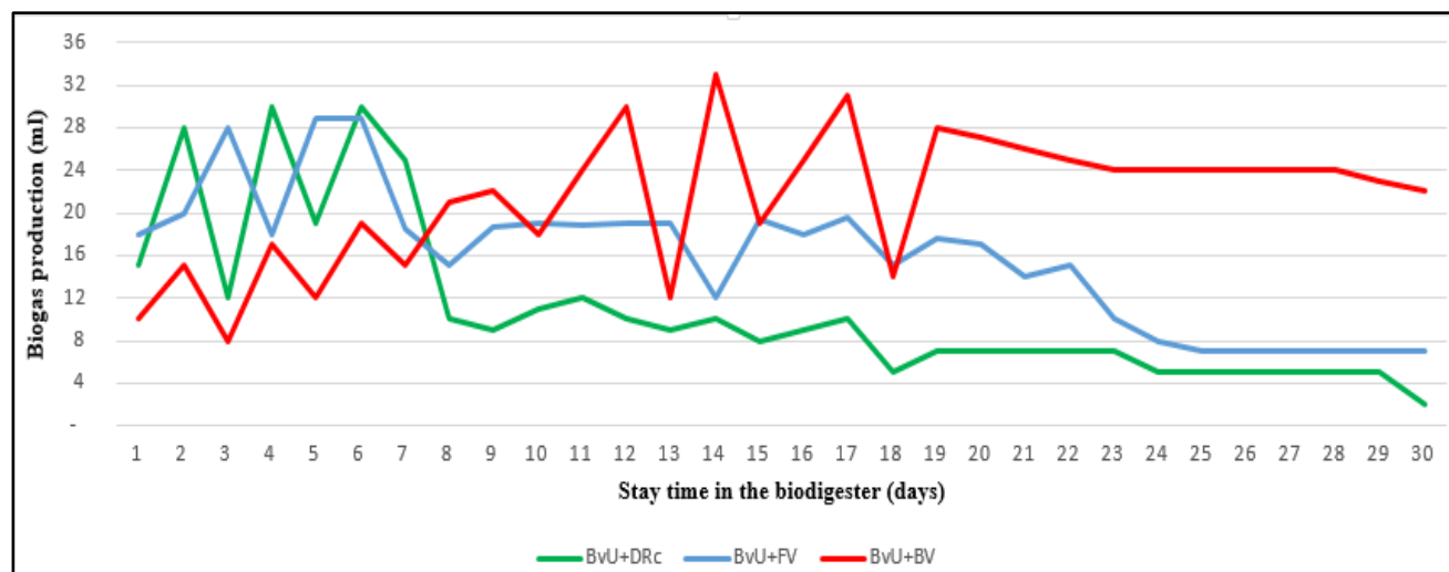
Figure 7. Biogas production by co-digestion under stirring per day at mesophilic temperature (40°C)
