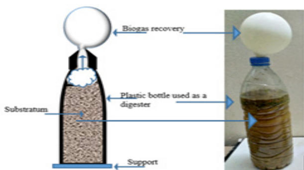
Figure 1. Diagram and photo of the digester
