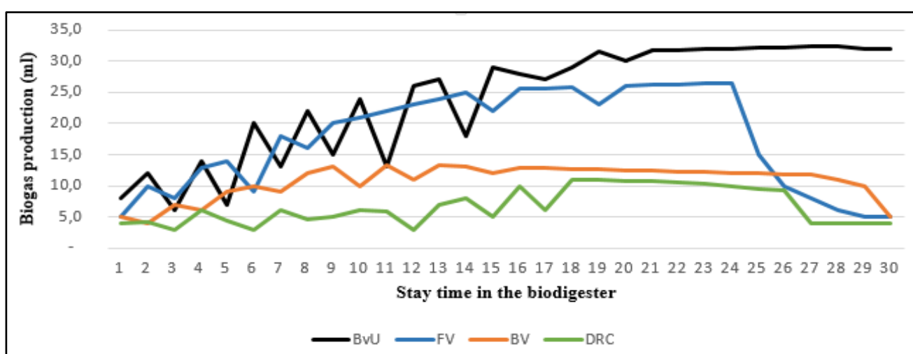
Figure 6. Production of biogas from a single substrate under stirring per day at mesophilic temperature (40°C)
