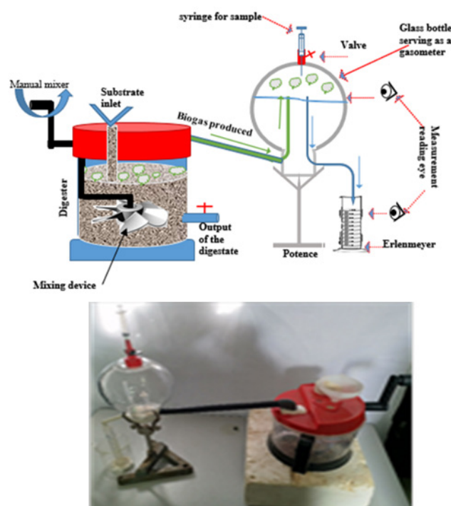
Figure 2. Diagram and photo of the reactor designed in the laboratory for the production of biogas
