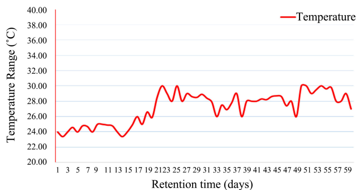
Figure 4. Temperature recorded for biogas production in Senegal.
