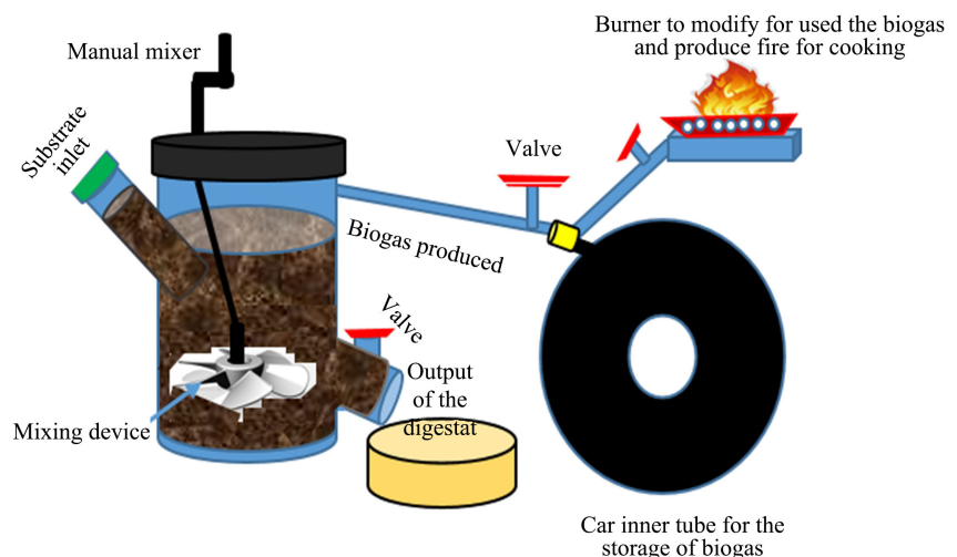
Figure 2. Diagram of the bio-digester.
